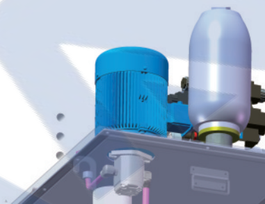
液压动力装置2 Hydraulic power plant 2
